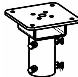
2-3/8" OD Tenon Mount Adaptor for Yoke Fixtures
